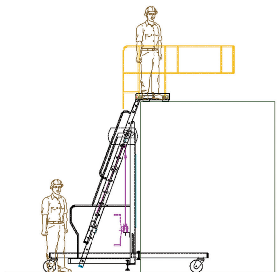
MK2 OR: Outrigger Mobile Step Unit illustration
