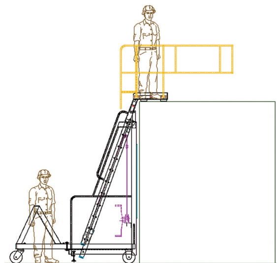
MK1 CB: Counter Balance Mobile Step Unit illustration
